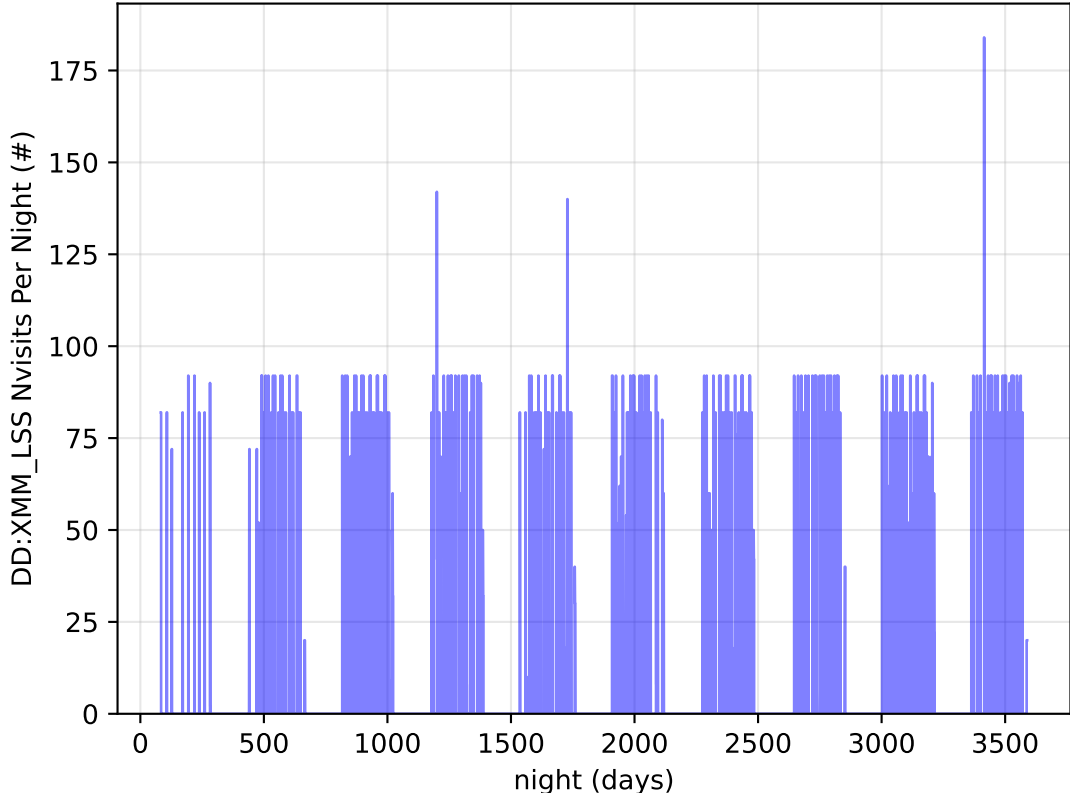
ddf_acor_sf15_lsf20_lsr10_v3.4_10yrs all bands: DD:XMM_LSS Nvisits Per Night
