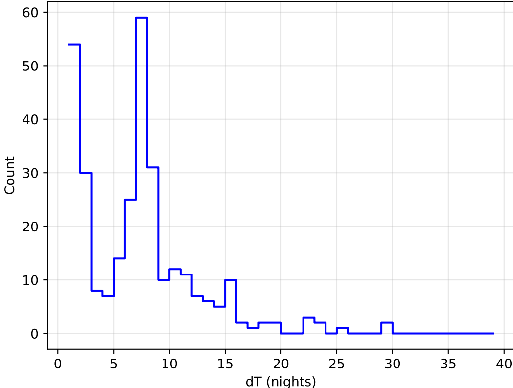
ddf_acor_sf15_lsf20_lsr10_v3.4_10yrs all bands: DD:XMM_LSS Delta Nights Histogram
