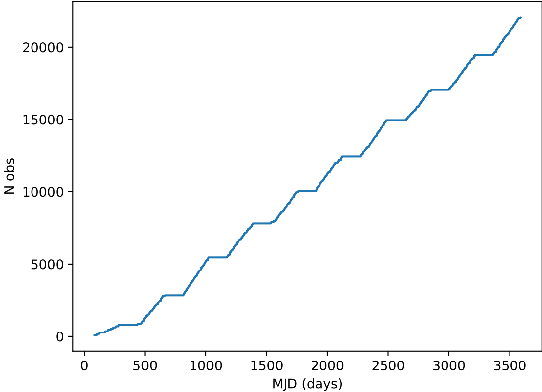
ddf_acor_sf15_lsf20_lsr10_v3.4_10yrs all bands: DD:XMM_LSS Cumulative NVisits
