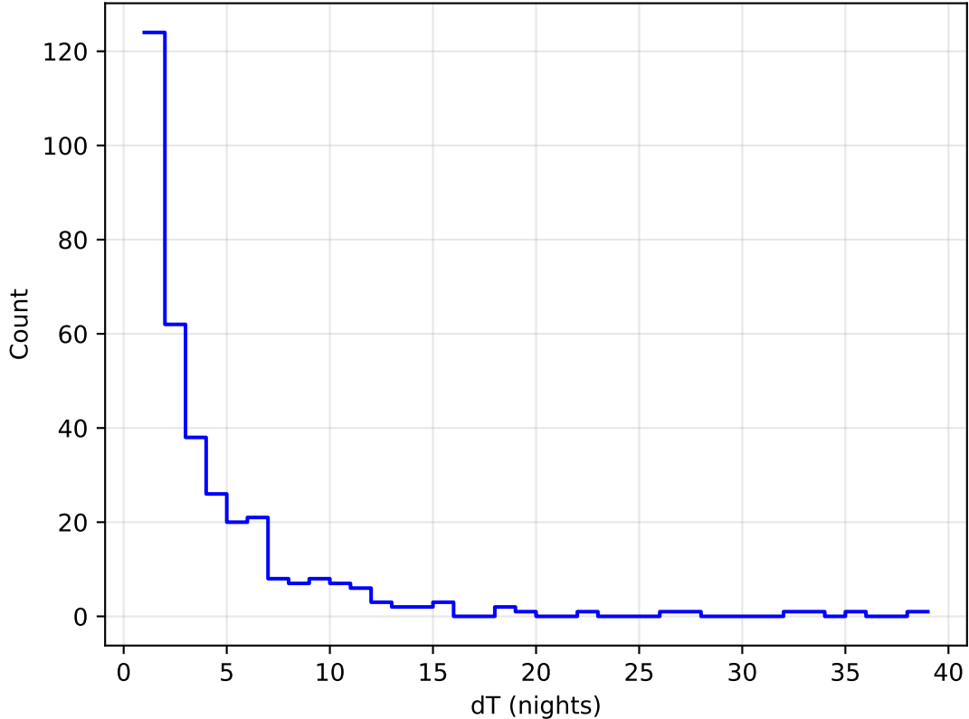
ddf_acor_sf15_lsf20_lsr10_v3.4_10yrs all bands: DD:WFD Delta Nights Histogram
