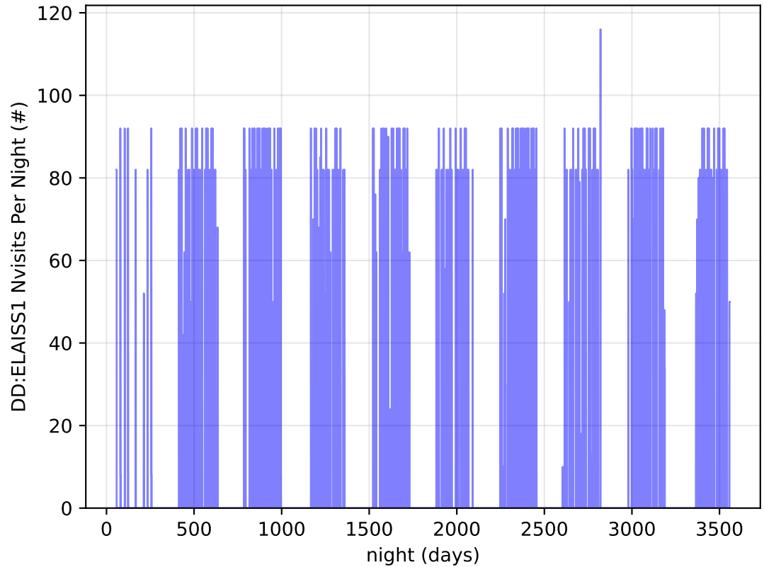
ddf_acor_sf15_lsf20_lsr10_v3.4_10yrs all bands: DD:ELAISS1 Nvisits Per Night
