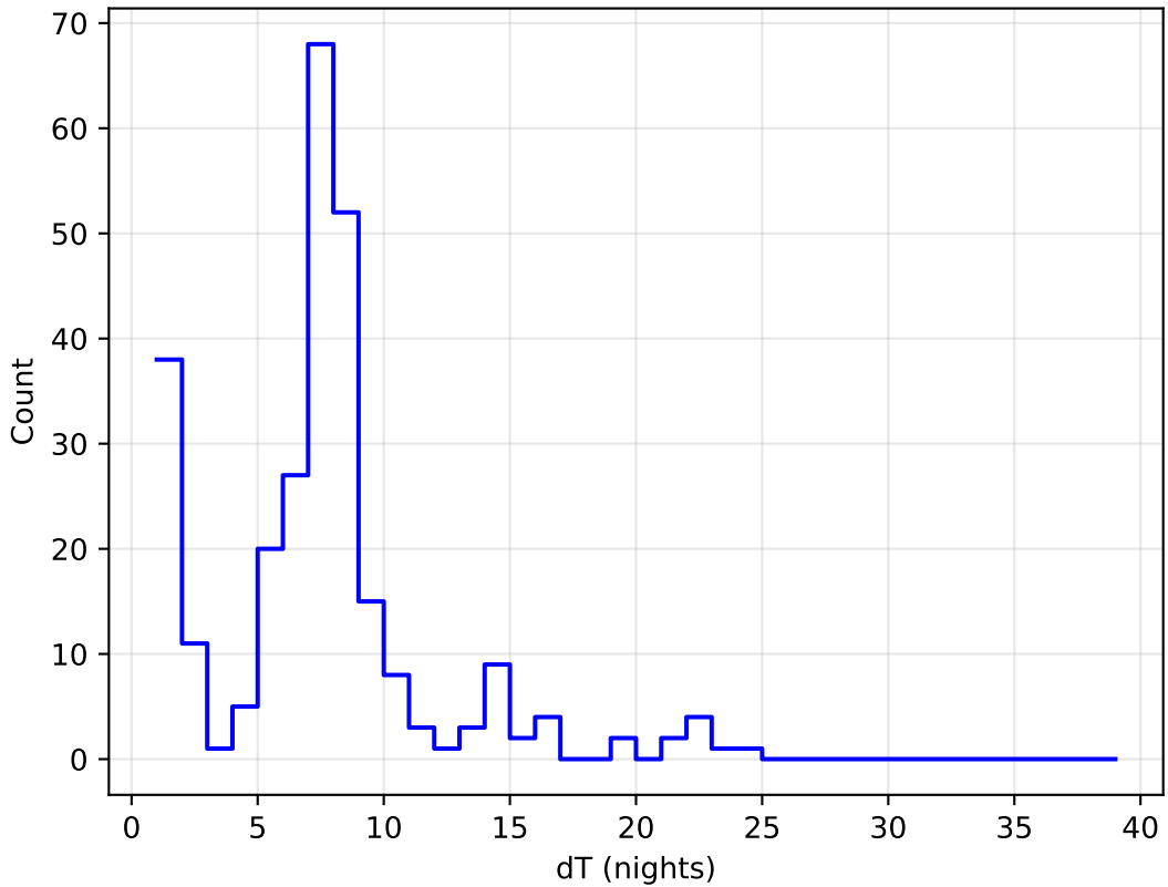
ddf_acor_sf15_lsf20_lsr10_v3.4_10yrs all bands: DD:ELAISS1 Delta Nights Histogram
