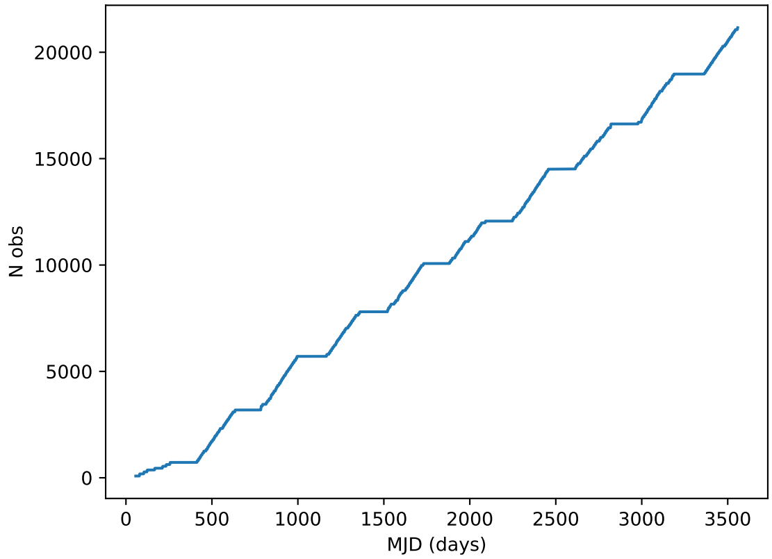
ddf_acor_sf15_lsf20_lsr10_v3.4_10yrs all bands: DD:ELAISS1 Cumulative NVisits
