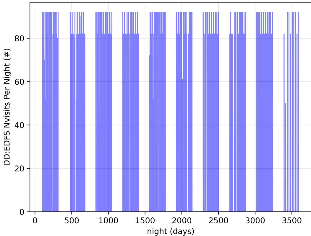
ddf_acor_sf15_lsf20_lsr10_v3.4_10yrs all bands: DD:EDFS Nvisits Per Night
