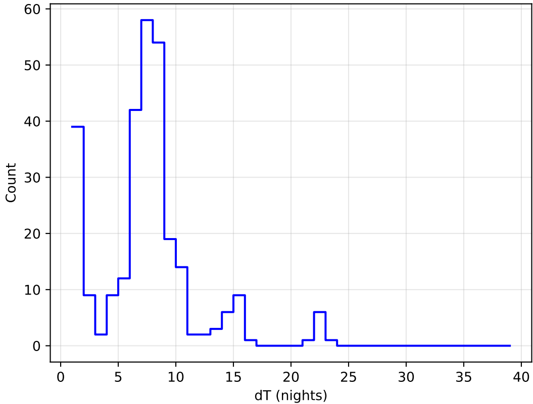
ddf_acor_sf15_lsf20_lsr10_v3.4_10yrs all bands: DD:ECDFS Delta Nights Histogram
