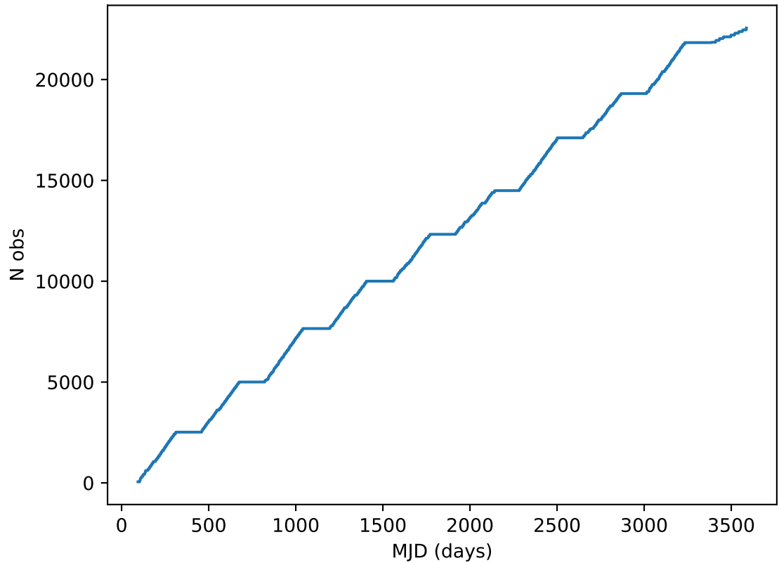
ddf_acor_sf15_lsf20_lsr10_v3.4_10yrs all bands: DD:ECDFS Cumulative NVisits
