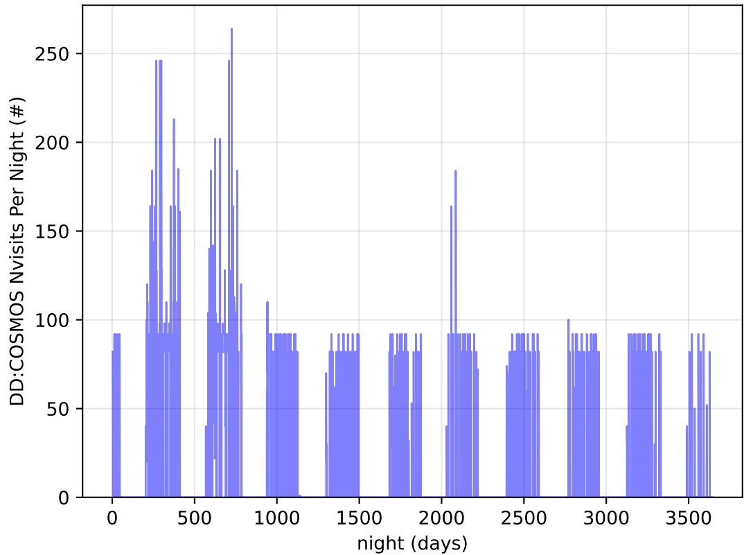
ddf_acor_sf15_lsf20_lsr10_v3.4_10yrs all bands: DD: COSMOS Nvisits Per Night
