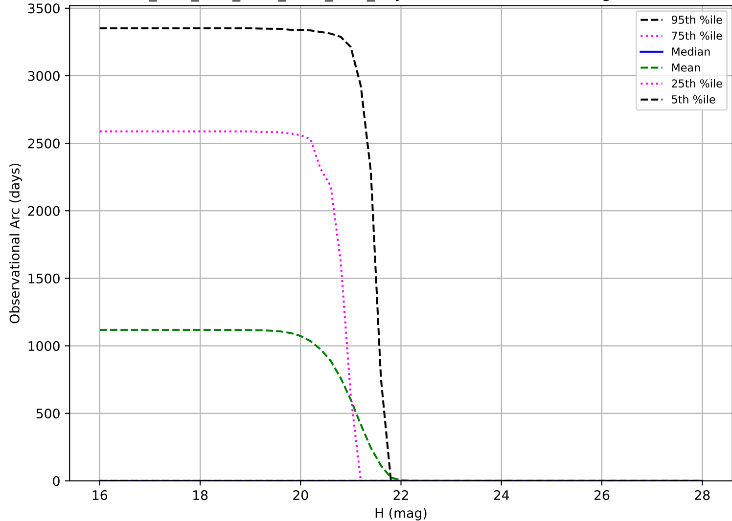
ddf_acor_sf10_lsf40_lsr50_v3.4_10yrs: Observational Arc Length Vatira
