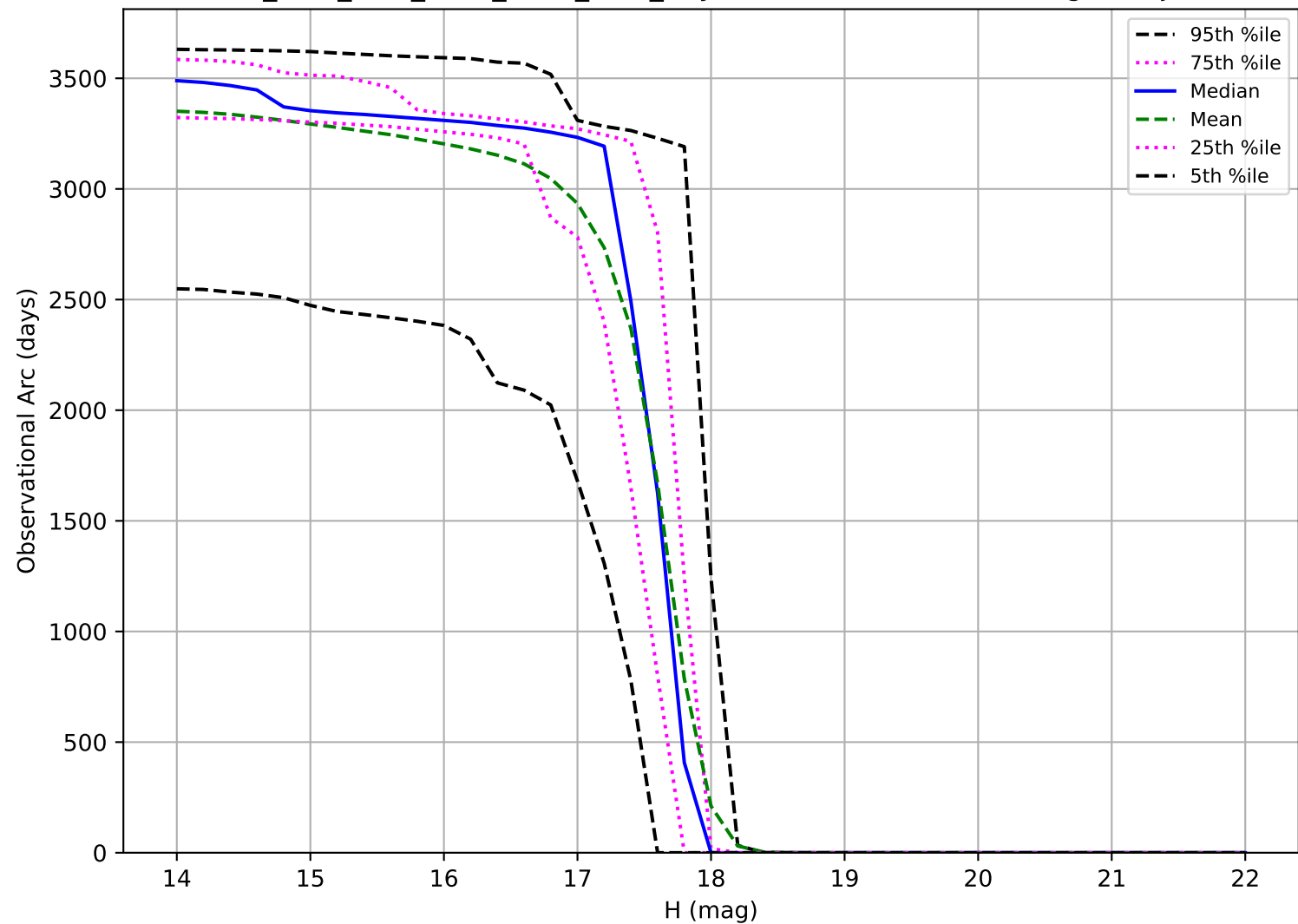
ddf_acor_sf10_lsf40_lsr50_v3.4_10yrs: Observational Arc Length Trojan
