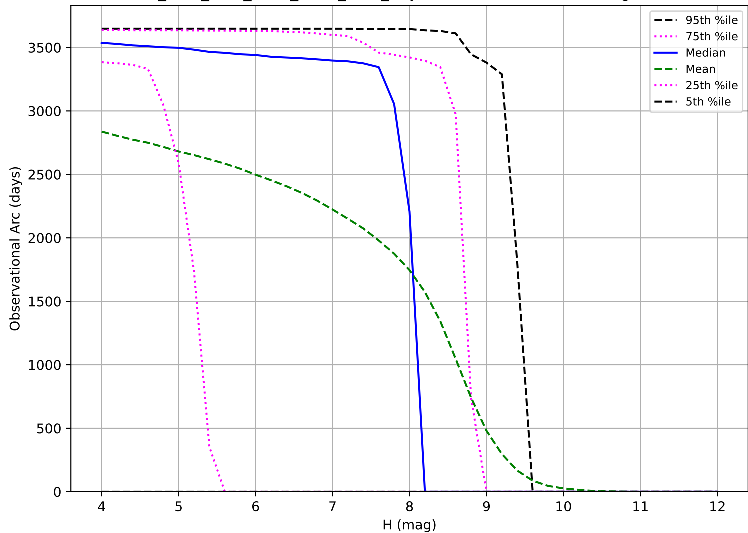
ddf_acor_sf10_Isf40_Isr50_v3.4_10yrs: Observational Arc Length TNO
