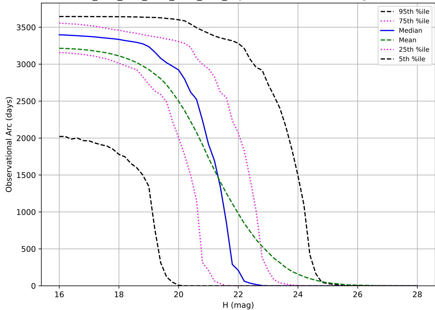
ddf_acor_sf10_lsf40_lsr50_v3.4_10yrs: Observational Arc Length PHA
