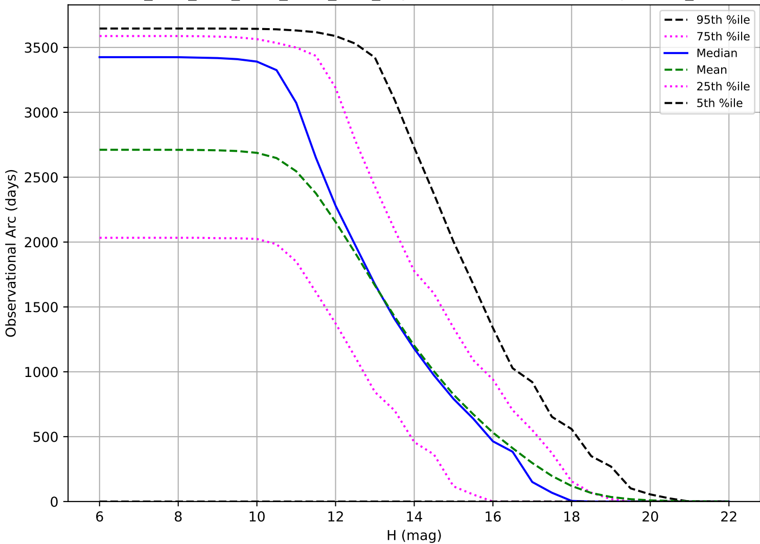
ddf_acor_sf10_lsf40_lsr50_v3.4_10yrs: Observational Arc Length OCC_r5
