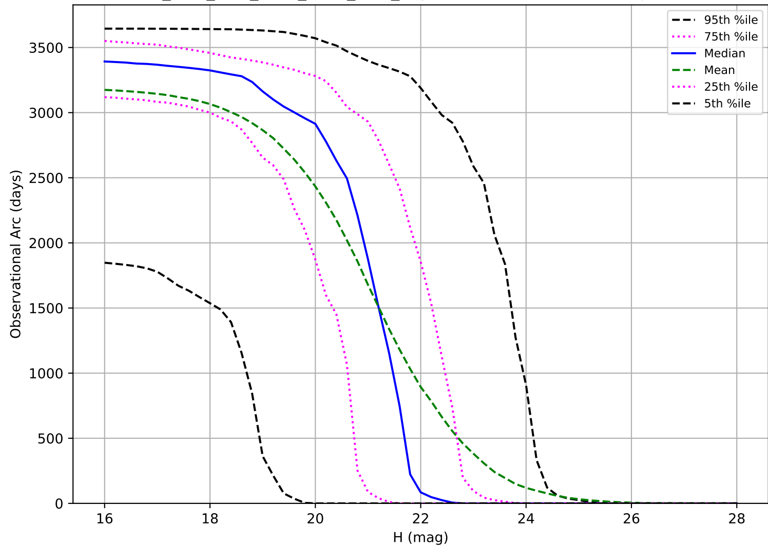
ddf_acor_sf10_lsf40_lsr50_v3.4_10yrs: Observational Arc Length NEO
