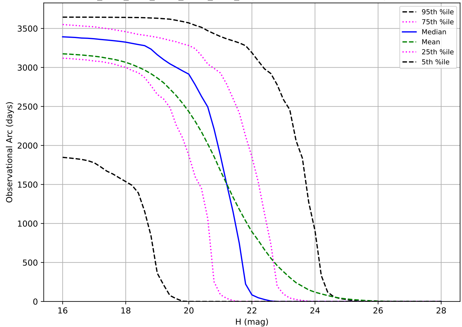
ddf_acor_sf10_lsf40_lsr50_v3.4_10yrs: Observational Arc Length NEO
