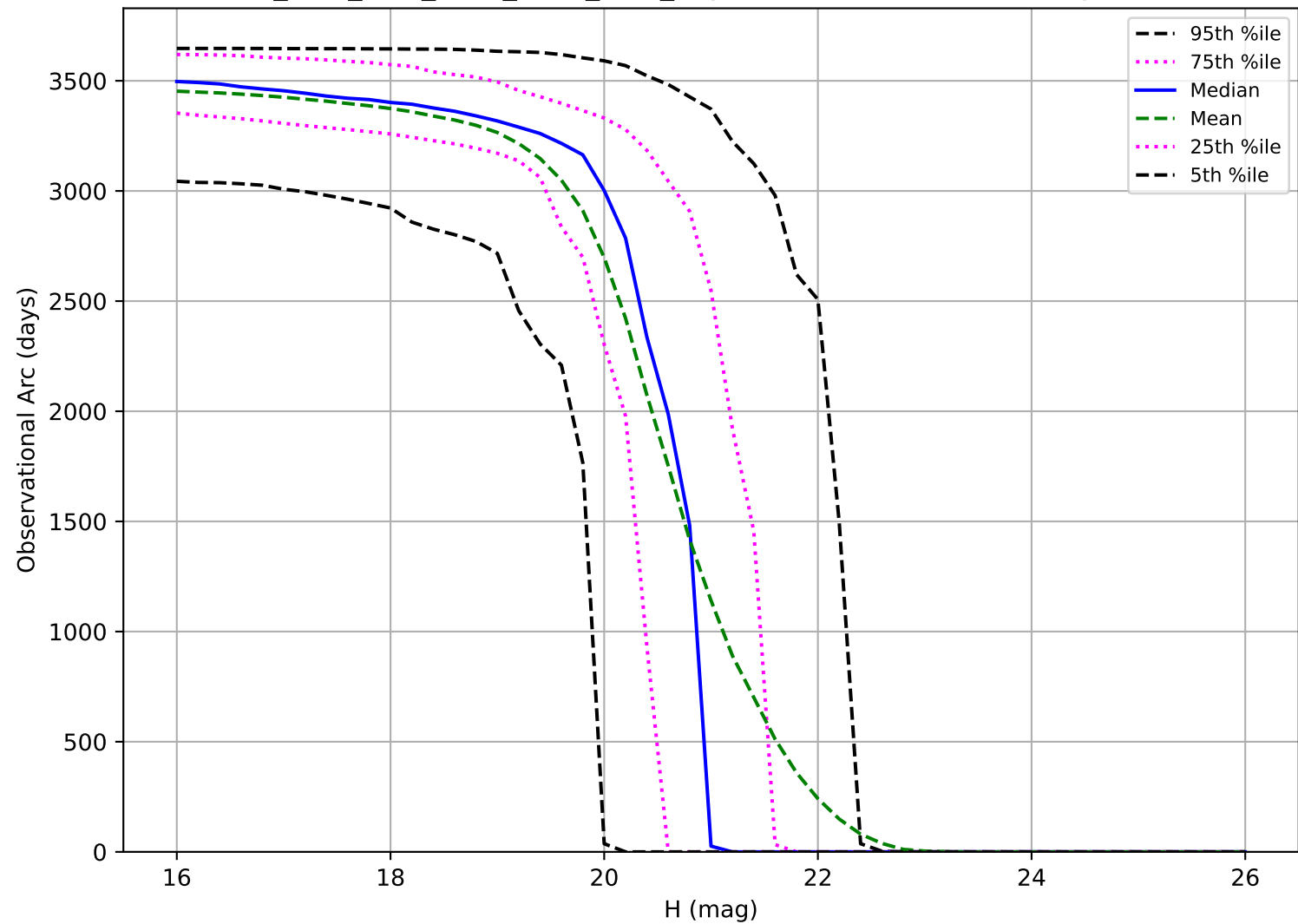
ddf_acor_sf10_lsf40_lsr50_v3.4_10yrs: Observational Arc Length MBA
