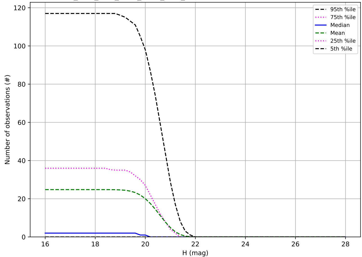
ddf_acor_sf10_lsf40_lsr50_v3.4_10yrs: Number of observations Vatira
