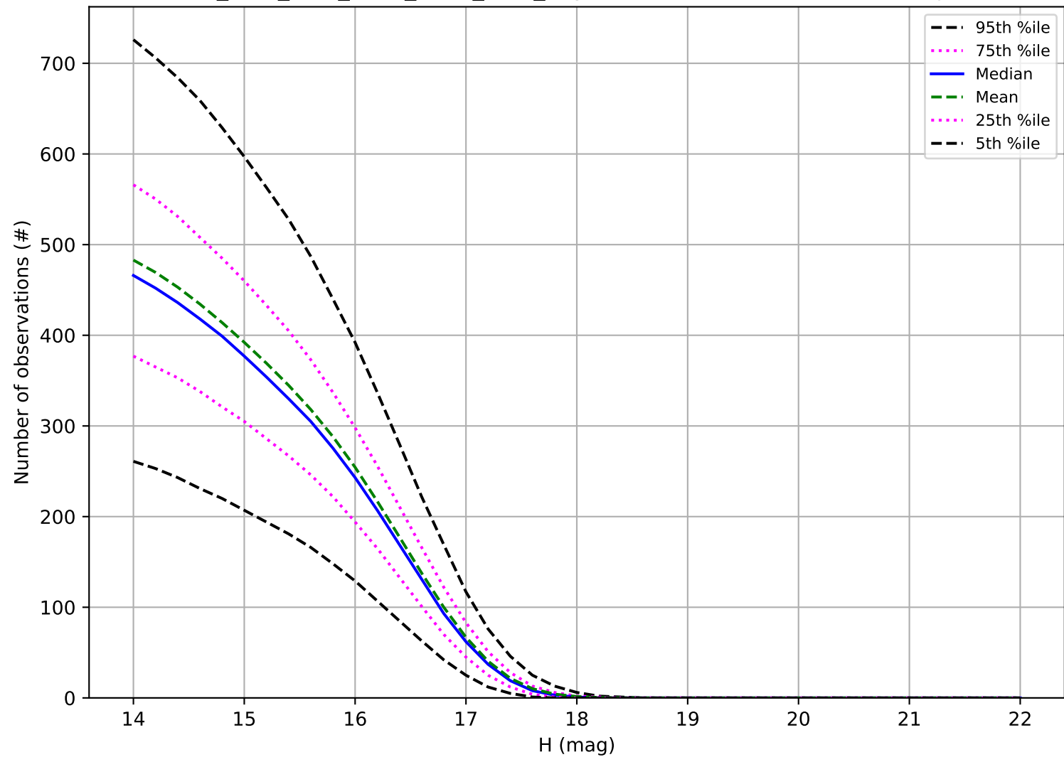
ddf_acor_sf10_lsf40_lsr50_v3.4_10yrs: Number of observations Trojan
