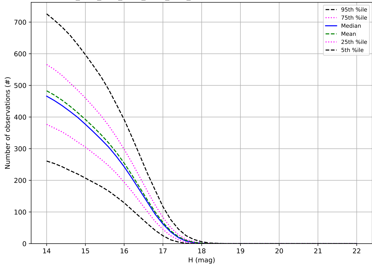
ddf_acor_sf10_lsf40_lsr50_v3.4_10yrs: Number of observations Trojan
