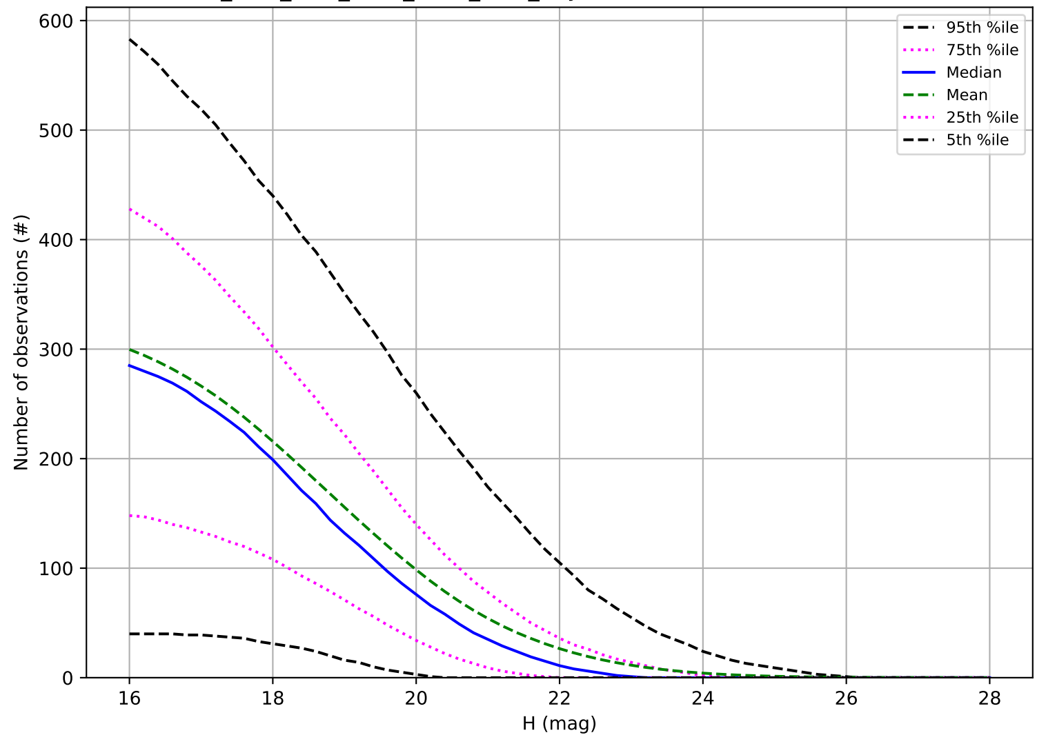
ddf_acor_sf10_lsf40_lsr50_v3.4_10yrs: Number of observations PHA
