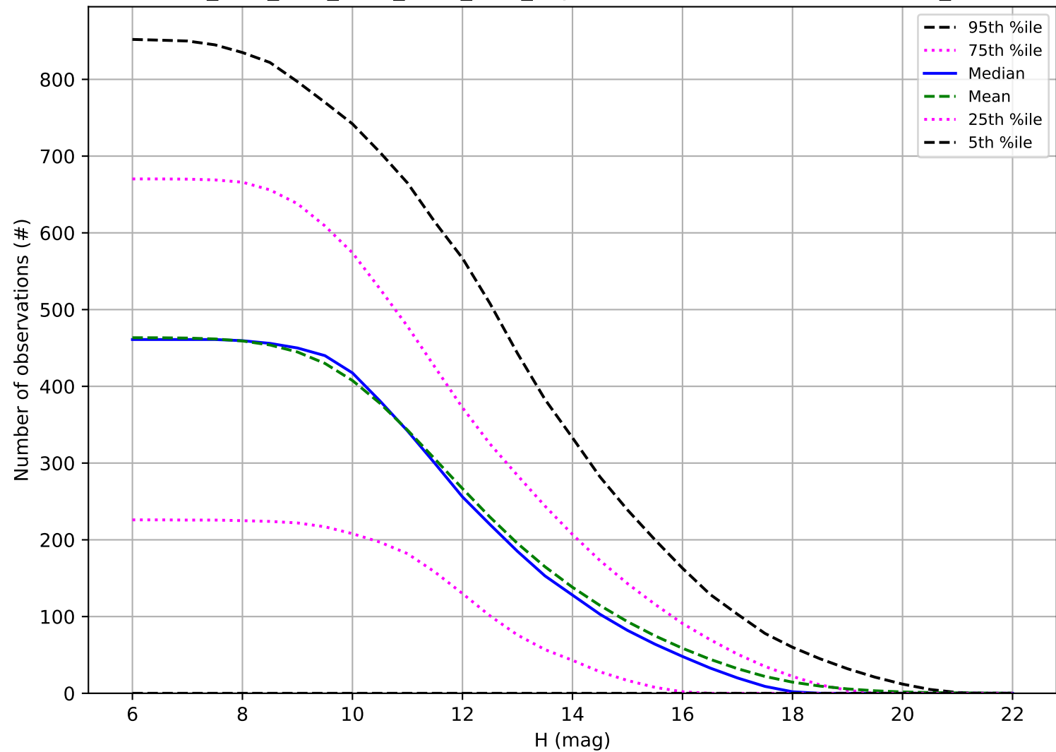
ddf_acor_sf10_lsf40_lsr50_v3.4_10yrs: Number of observations OCC_r5
