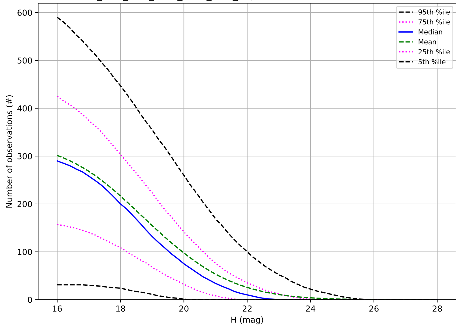
ddf_acor_sf10_lsf40_lsr50_v3.4_10yrs: Number of observations NEO
