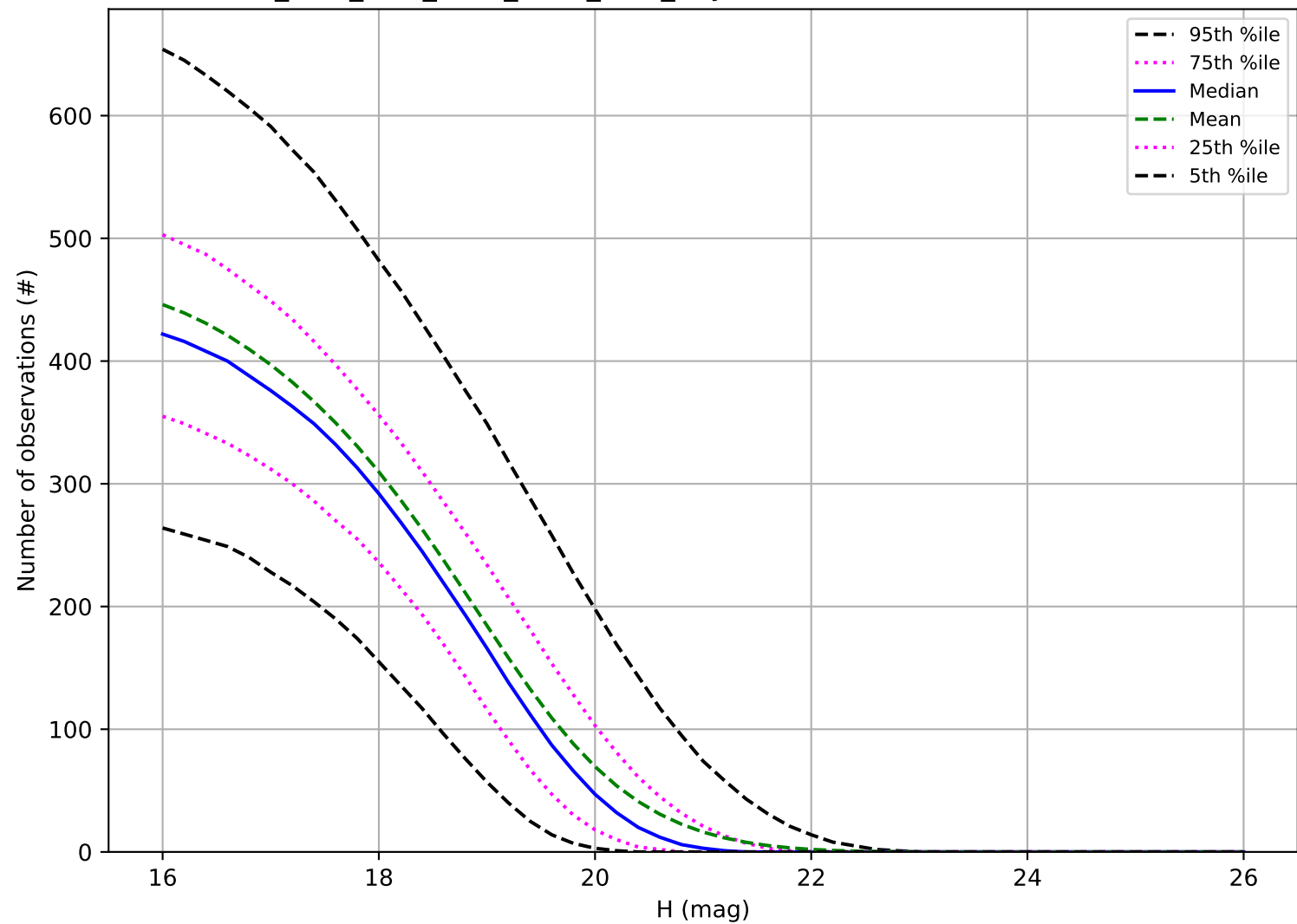
ddf_acor_sf10_lsf40_lsr50_v3.4_10yrs: Number of observations MBA
