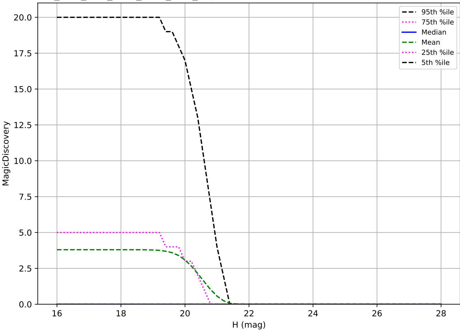
ddf_acor_sf10_lsf40_lsr50_v3.4_10yrs: Vatira 6 detections in 60 nights detection loss
