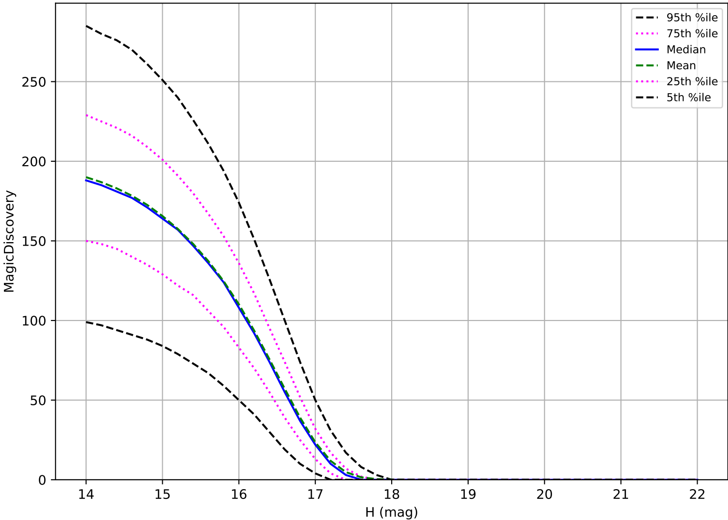
ddf_acor_sf10_lsf40_lsr50_v3.4_10yrs: Trojan 6 detections in 60 nights detection loss
