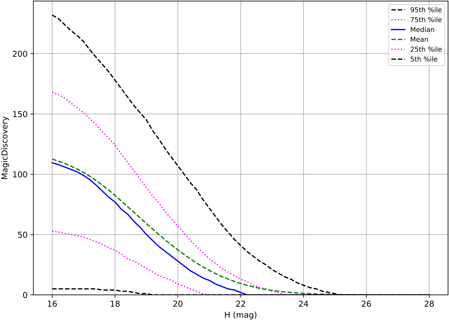
ddf_acor_sf10_lsf40_lsr50_v3.4_10yrs: NEO 6 detections in 60 nights detection loss
