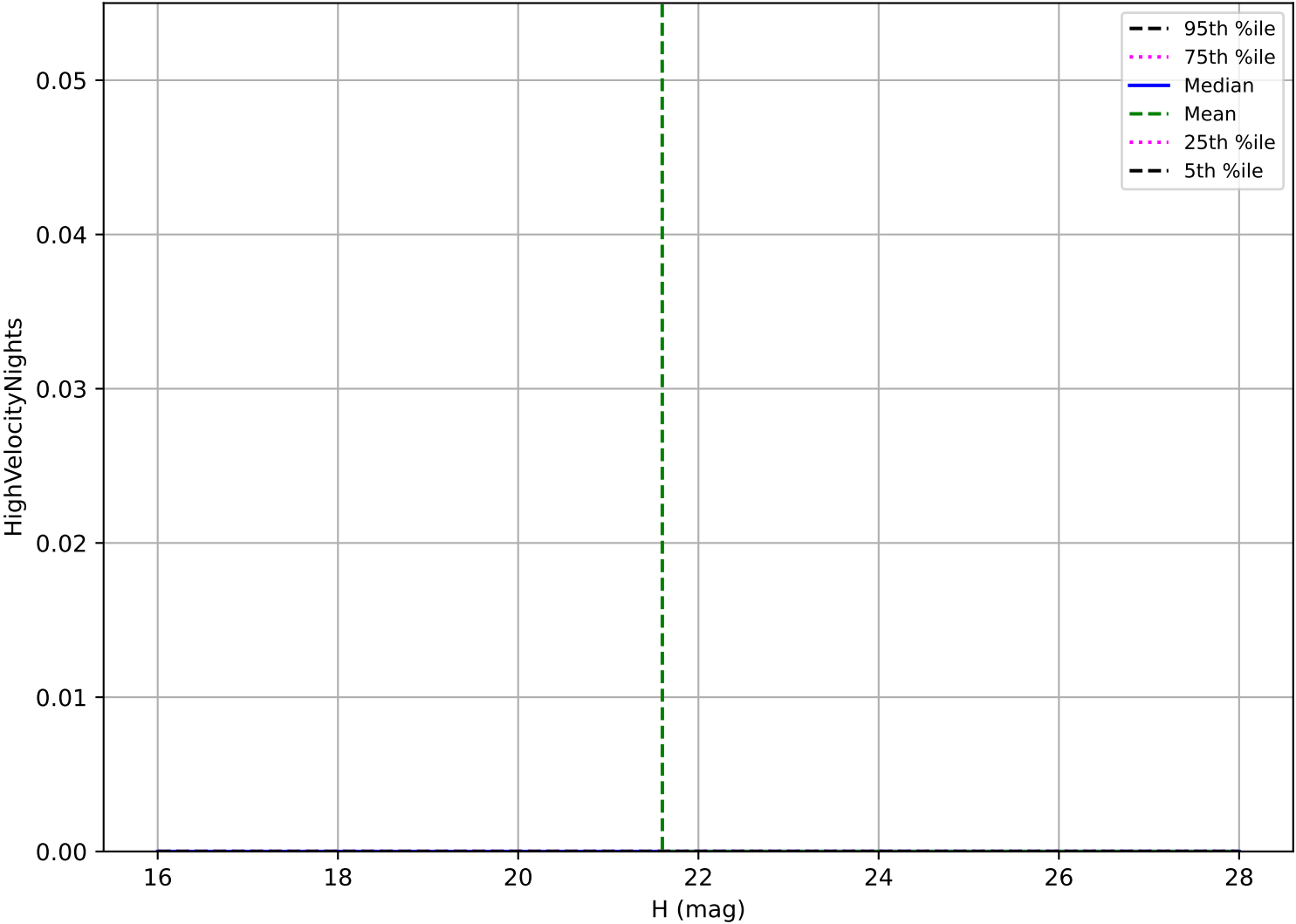
ddf_acor_sf10_lsf40_lsr50_v3.4_10yrs: Vatira High velocity pair detection loss
