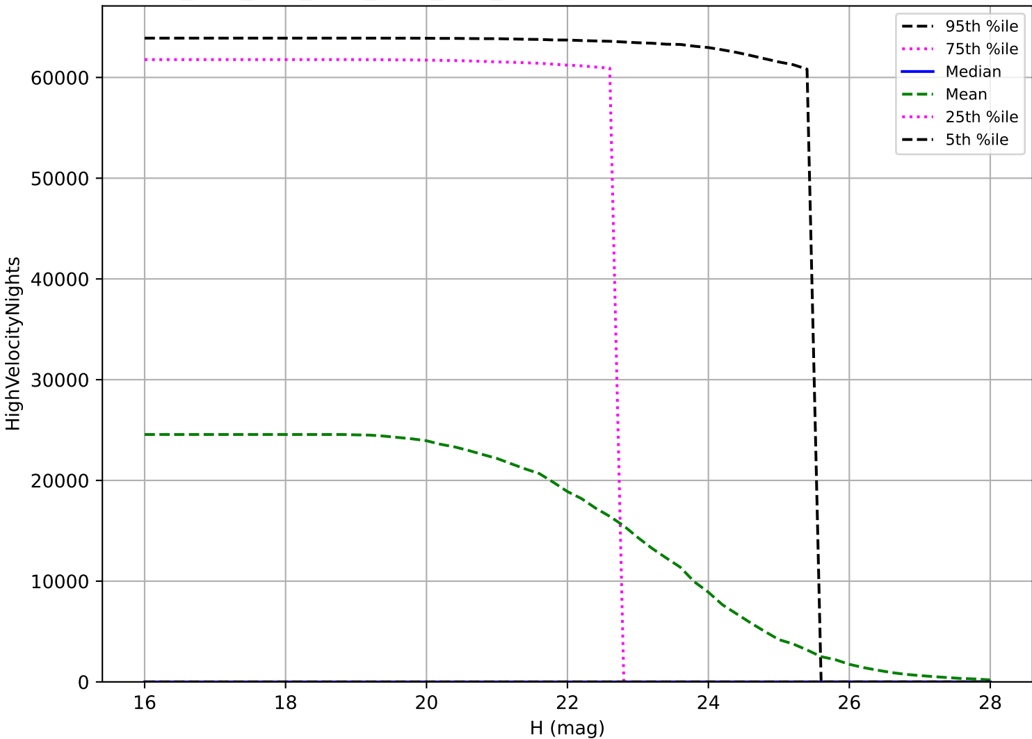
ddf_acor_sf10_lsf40_lsr50_v3.4_10yrs: PHA High velocity pair detection loss
