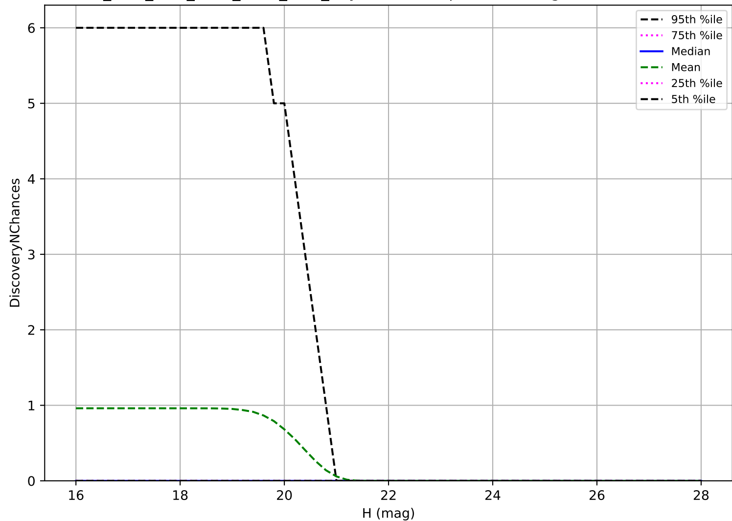
ddf_acor_sf10_lsf40_lsr50_v3.4_10yrs: Vatira 3 pairs in 15 nights detection loss
