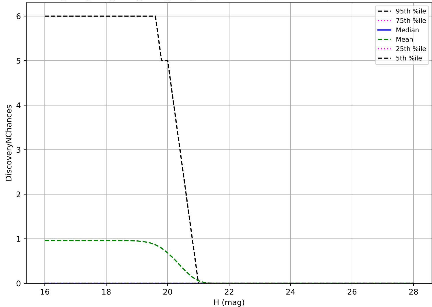
ddf_acor_sf10_lsf40_lsr50_v3.4_10yrs: Vatira 3 pairs in 15 nights detection loss
