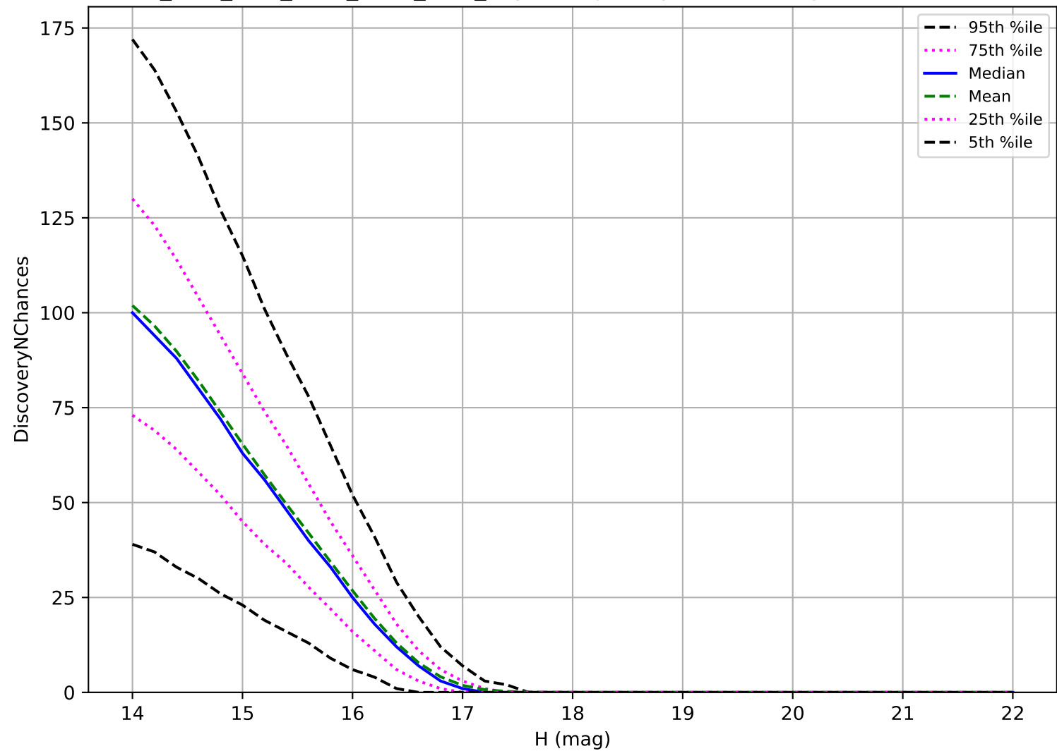
ddf_acor_sf10_lsf40_lsr50_v3.4_10yrs: Trojan 3 pairs in 15 nights detection loss
