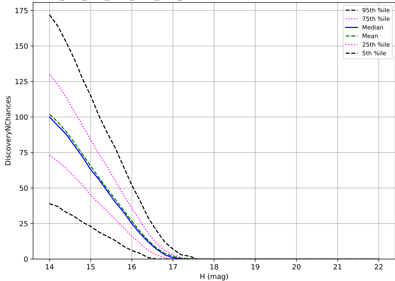
ddf_acor_sf10_lsf40_lsr50_v3.4_10yrs: Trojan 3 pairs in 15 nights detection loss
