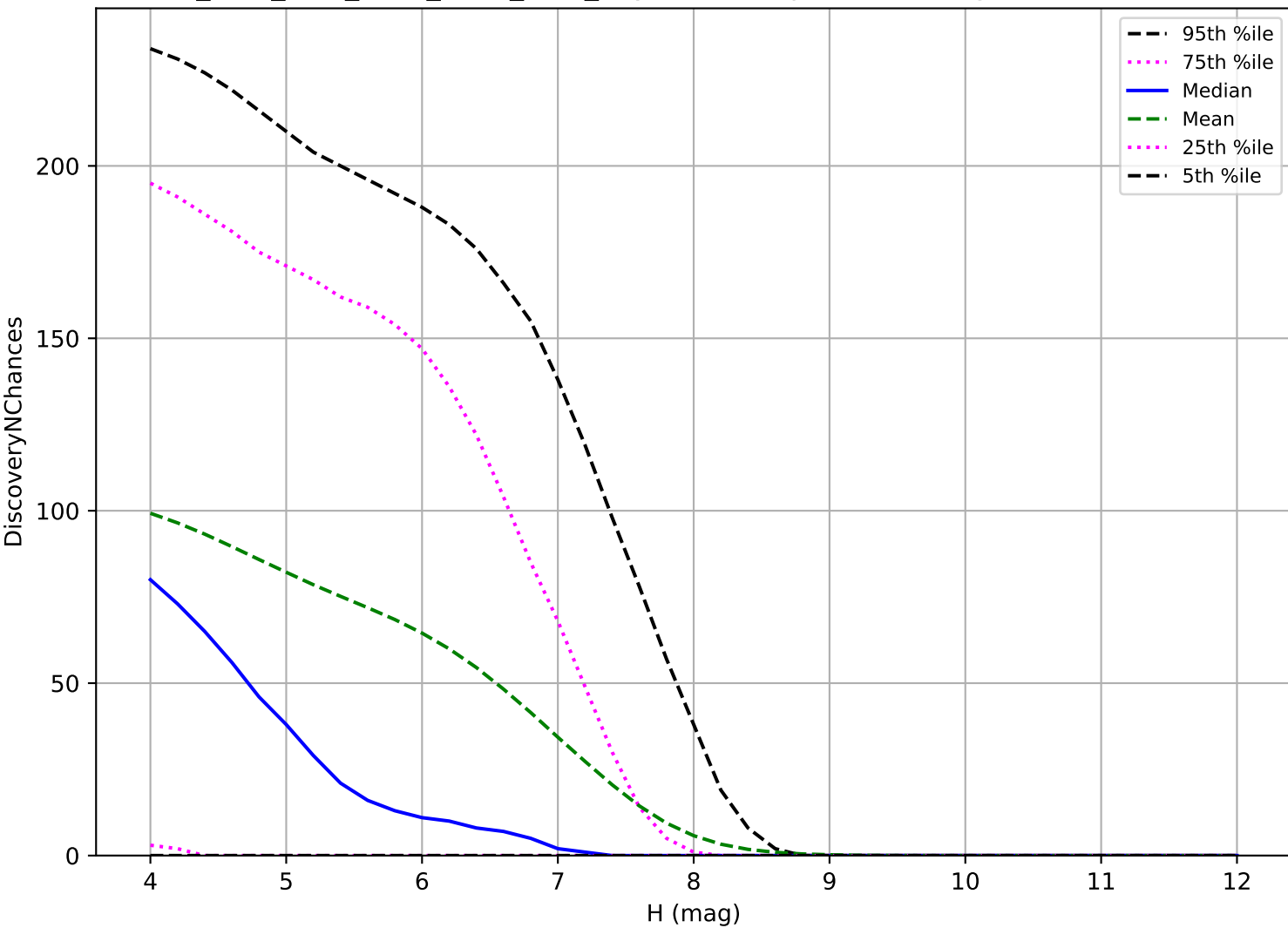
ddf_acor_sf10_lsf40_lsr50_v3.4_10yrs: TNO 3 pairs in 15 nights detection loss
