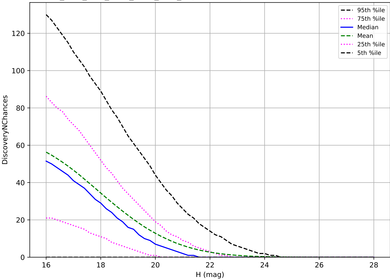
ddf_acor_sf10_lsf40_lsr50_v3.4_10yrs: NEO 3 pairs in 15 nights detection loss
