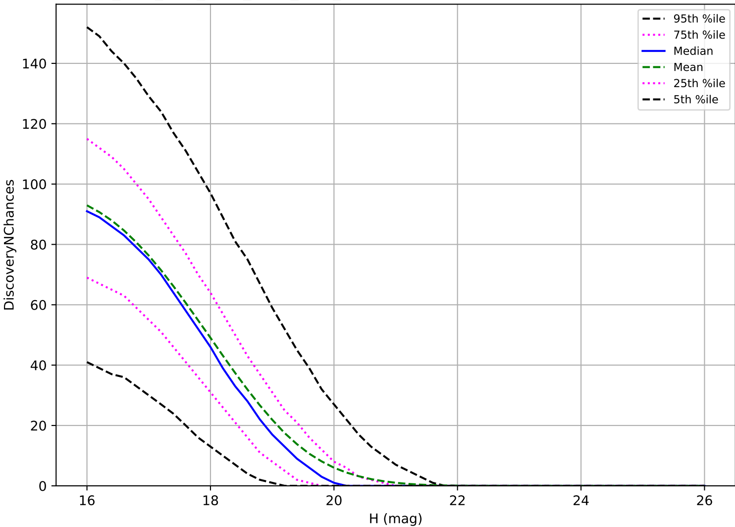
ddf_acor_sf10_lsf40_lsr50_v3.4_10yrs: MBA 3 pairs in 15 nights detection loss
