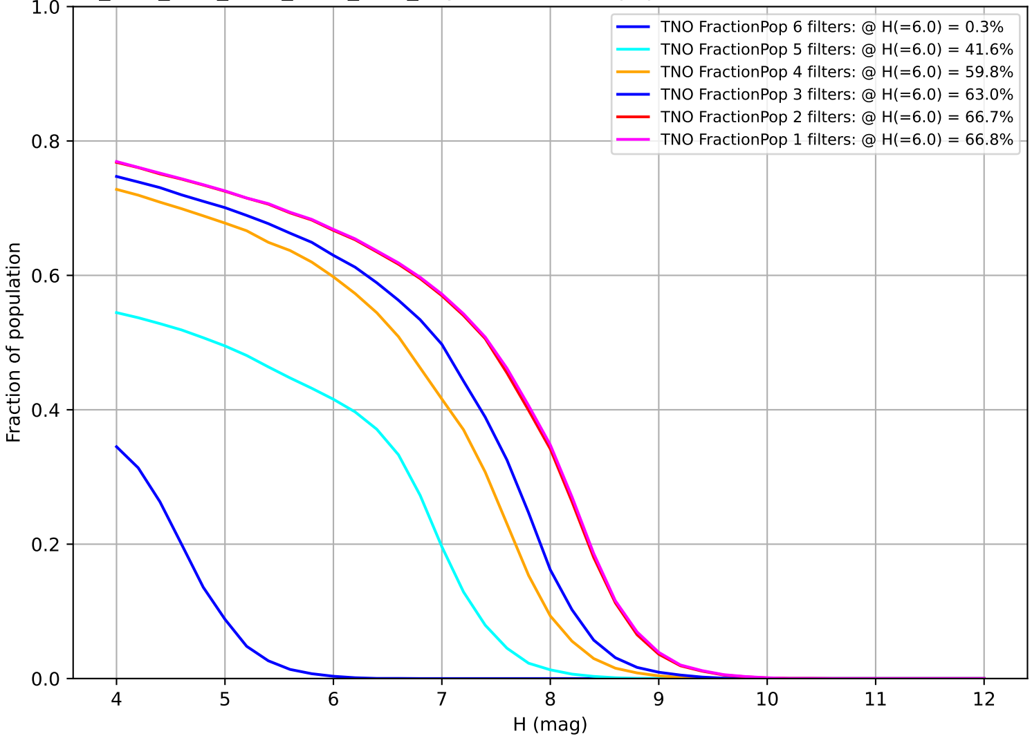
ddf_acor_sf10_lsf40_lsr50_v3.4_10yrs: Fraction of population with colors in X filters TNO
