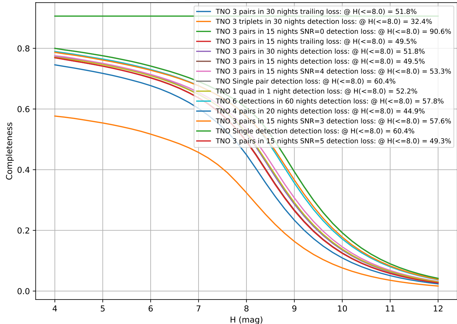
ddf_acor_sf10_lsf40_lsr50_v3.4_10yrs: CumulativeCompleteness
