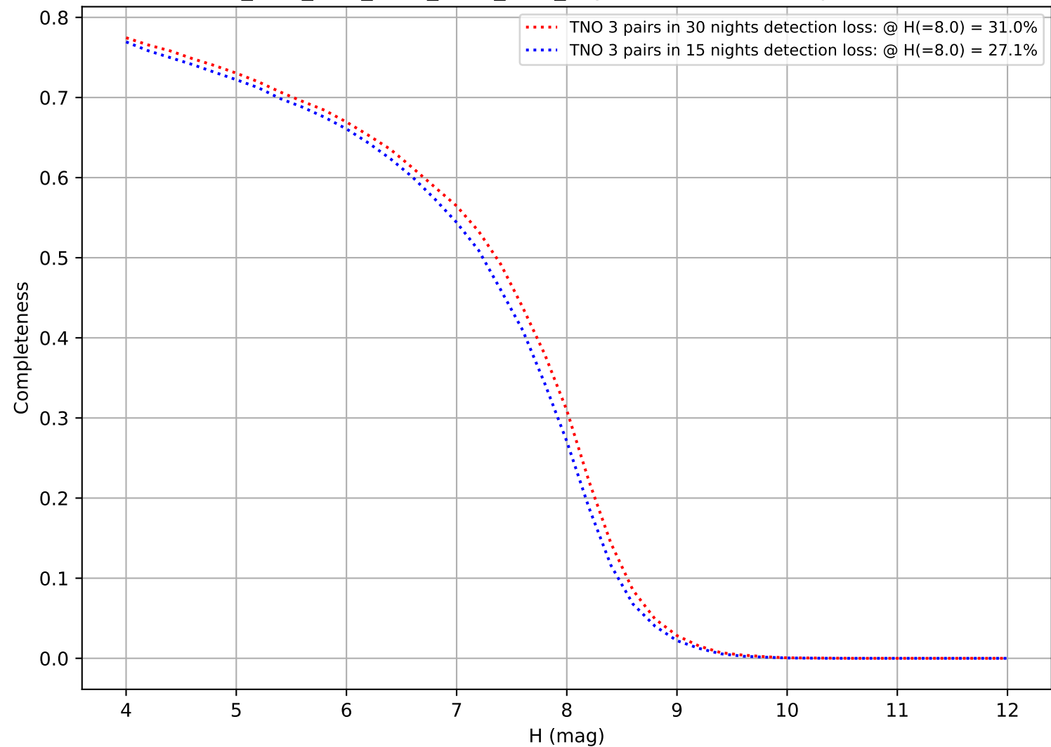
ddf_acor_sf10_lsf40_lsr50_v3.4_10yrs: DifferentialCompleteness
