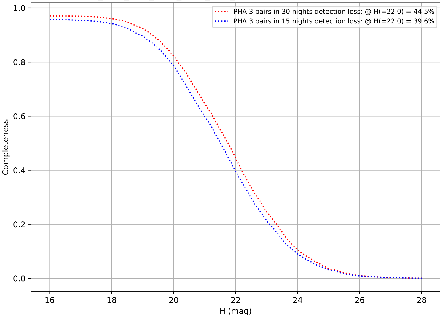
ddf_acor_sf10_lsf40_lsr50_v3.4_10yrs: DifferentialCompleteness
