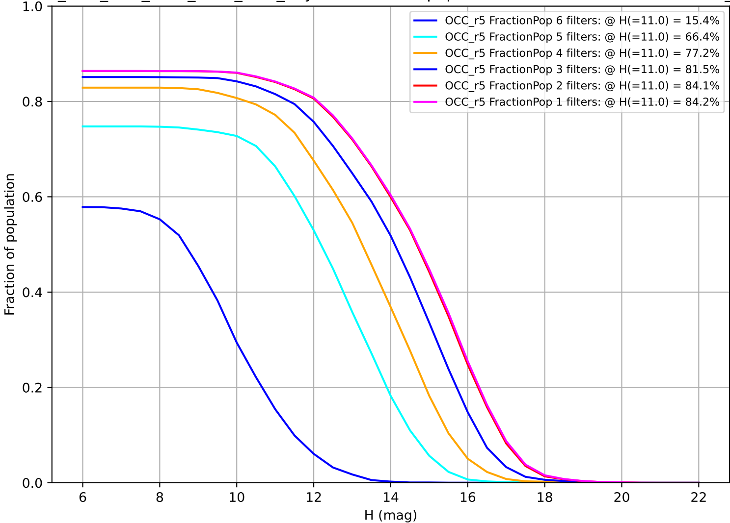
ddf_acor_sf10_lsf40_lsr50_v3.4_10yrs: Fraction of population with colors in X filters OCC_r5
