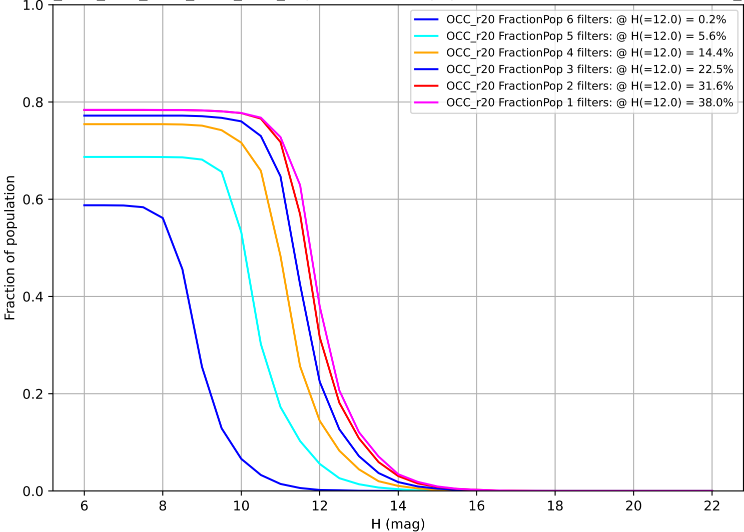
ddf_acor_sf10_lsf40_lsr50_v3.4_10yrs: Fraction of population with colors in X filters OCC_r20
