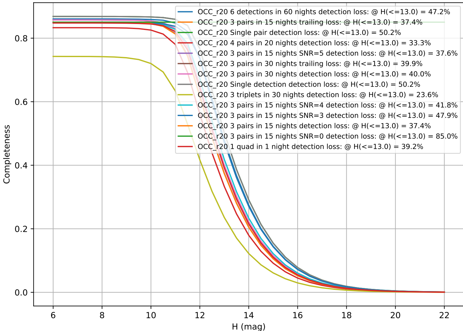
ddf_acor_sf10_lsf40_lsr50_v3.4_10yrs: CumulativeCompleteness
