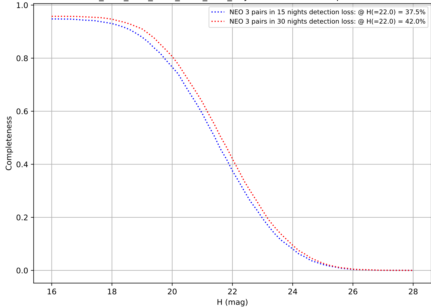
ddf_acor_sf10_lsf40_lsr50_v3.4_10yrs: DifferentialCompleteness
