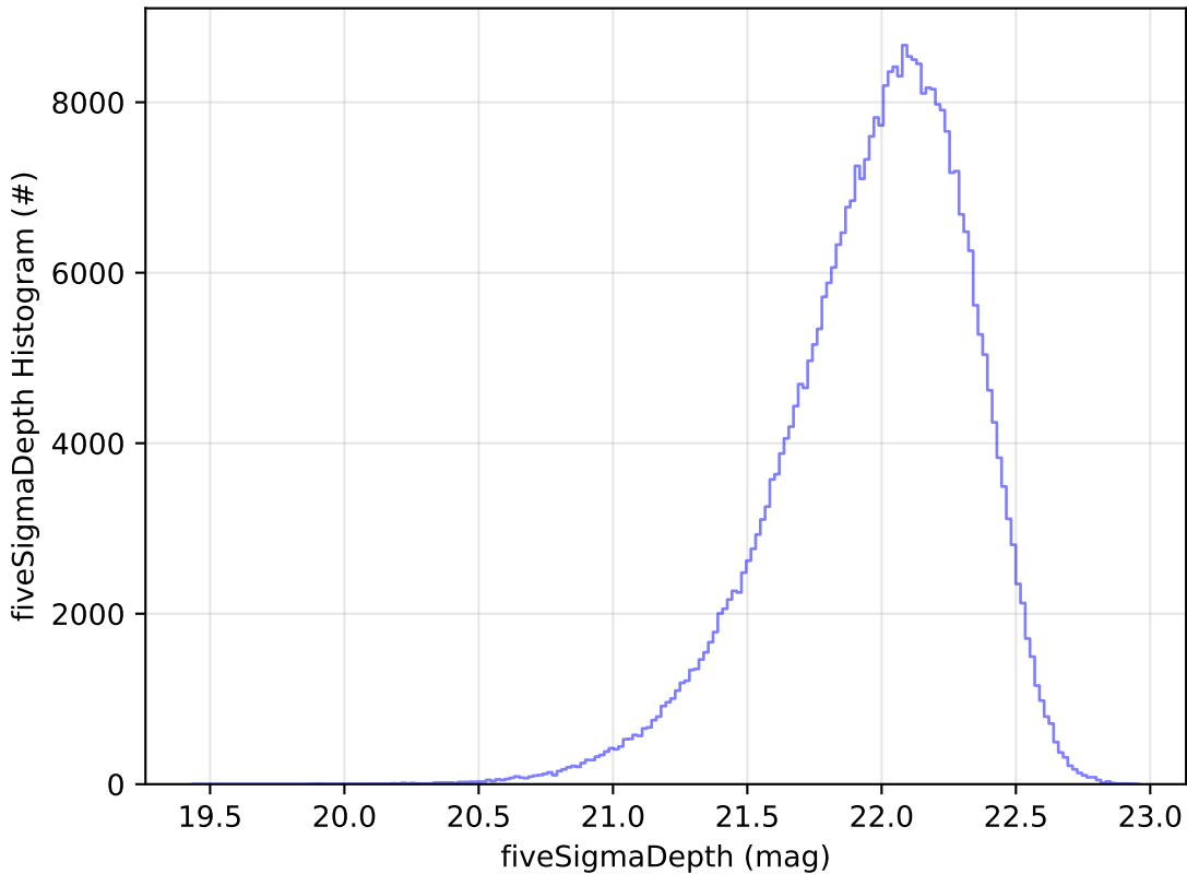
ddf_acor_sf10_lsf40_lsr50_v3.4_10yrs y: fiveSigmaDepth Histogram
