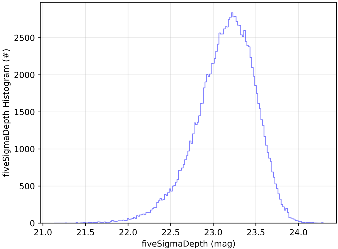
ddf_acor_sf10_lsf40_lsr50_v3.4_10yrs u: fiveSigmaDepth Histogram
