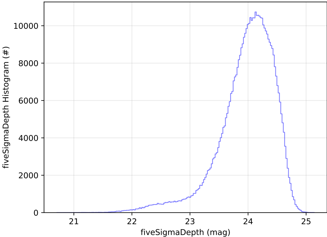
ddf_acor_sf10_lsf40_lsr50_v3.4_10yrs r: fiveSigmaDepth Histogram
