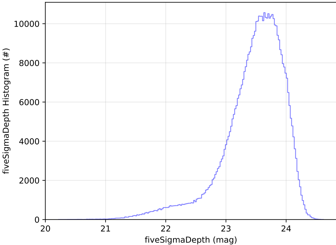
ddf_acor_sf10_lsf40_lsr50_v3.4_10yrs i: fiveSigmaDepth Histogram
