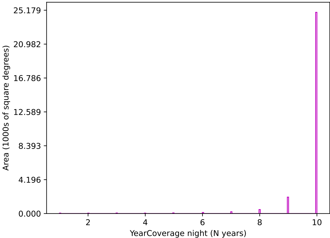
ddf_acor_sf10_lsf40_lsr50_v3.4_10yrs z band: YearCoverage night
