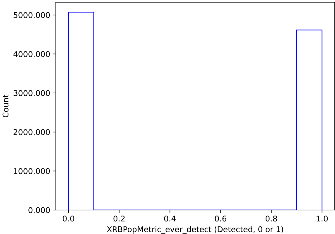
ddf_acor_sf10_lsf40_lsr50_v3.4_10yrs : XRBPoMetric_ever_detect
