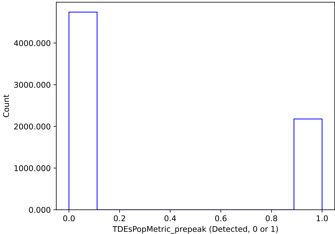
ddf_acor_sf10_lsf40_lsr50_v3.4_10yrs : TDEsPopMetric_prepeak
