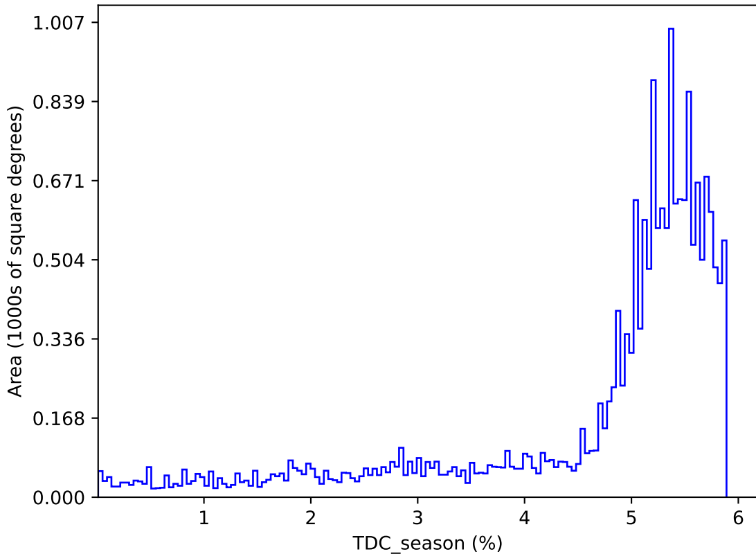
ddf_acor_sf10_lsf40_lsr50_v3.4_10yrs : TDC_season
